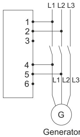
Electrical connections for a) Un 380V b) 440 V
